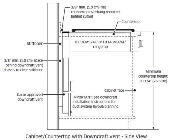
Cabinet/Countertop with Downdraft vent - Side View
