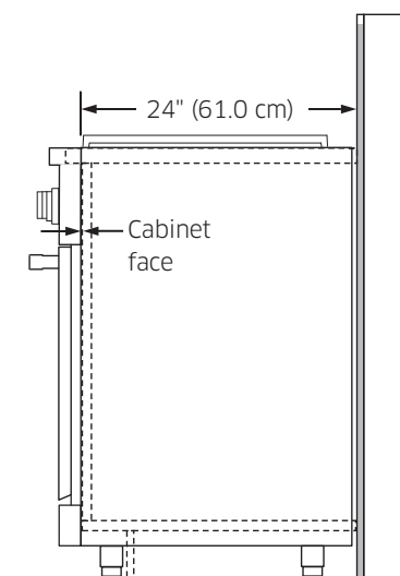
Range Installed
