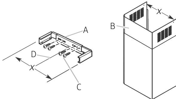
A. Vent cover bracket assembly B. Upper vent cover C. 4 - 4.2 x 8 mm screws D. Centerline
