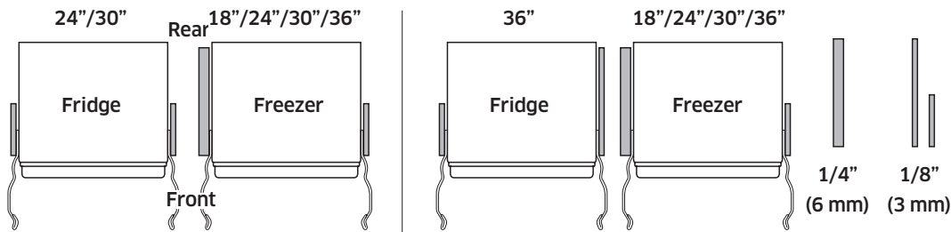
Top View
