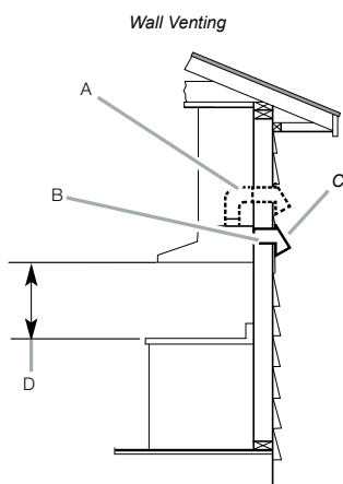
A. 6" (15.2 cm) round vent + 90° elbow B. 3/4" x 10" (8.25 x 25.4 cm) rectangular vent C. Wall cap D. Installation height
