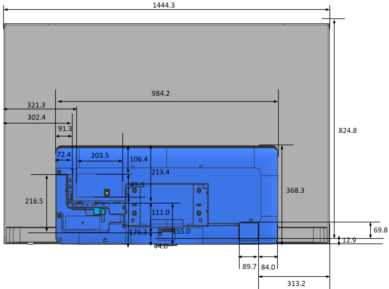
S90C 65" Cover and Rear-View Dimensions
