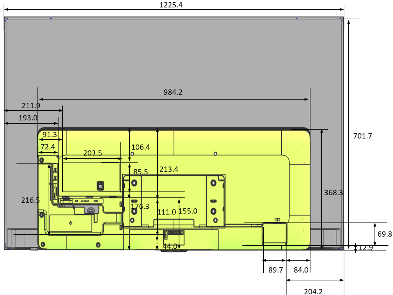
S90C 55" Cover and Rear-View Dimensions
