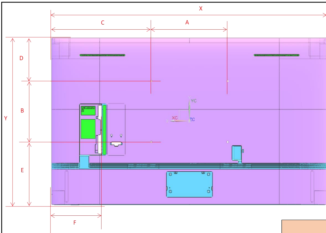
QN85C Cover and Rear-View Dimensions
