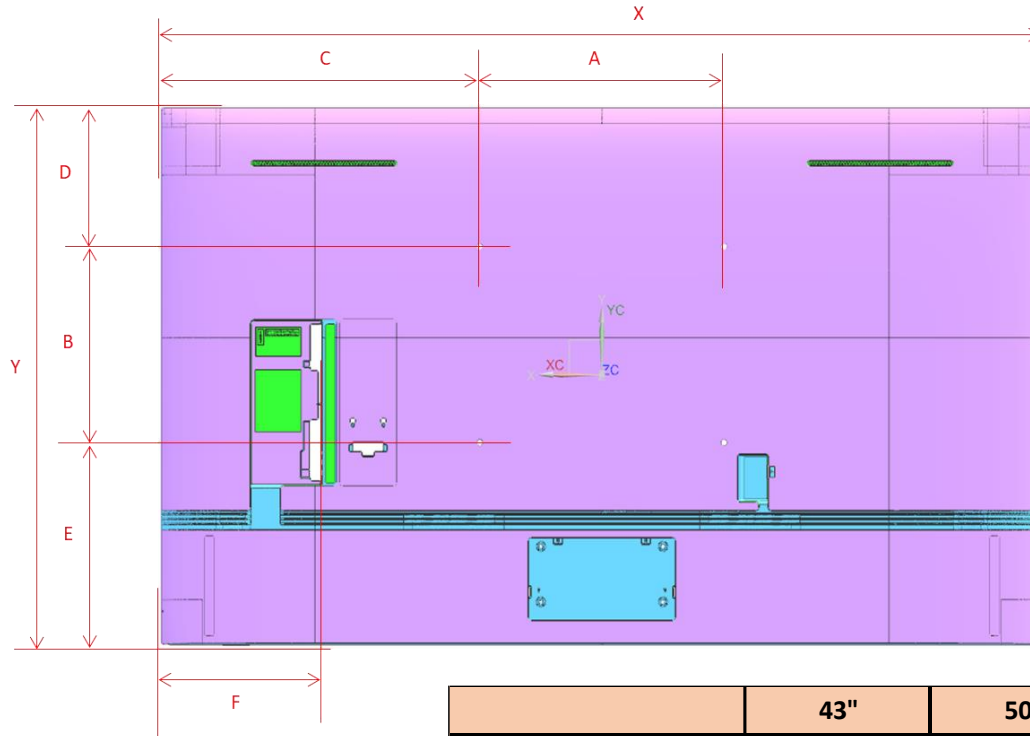
QN90C Cover and Rear-View Dimensions
